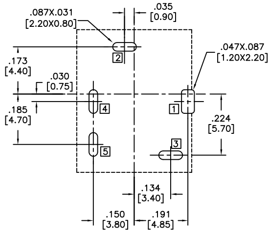
RECOMMENDED PCB LAYOUT (Copper-sided view)
