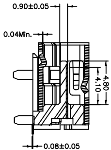
SECTION S-S SCALE 1:1
