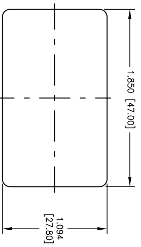
PANEL CUT-OUT
