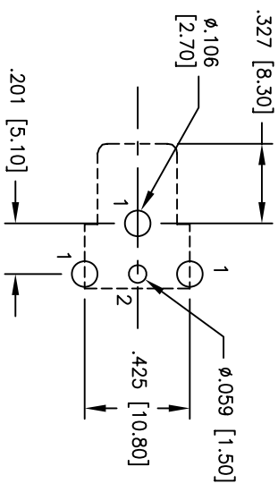
PCB LAYOUT
